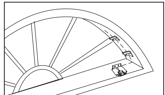
Inside Mount
