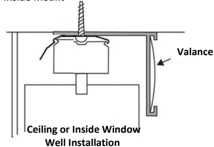
Inside Mount
